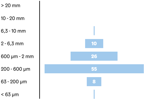
Figure 4 Results of particle size distribution based on weight and volume on soft green waste biochar
